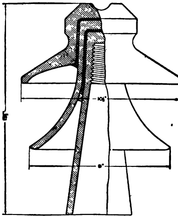
FIG. 9. SHAWINIGAN-FALLS INSULATOR.
